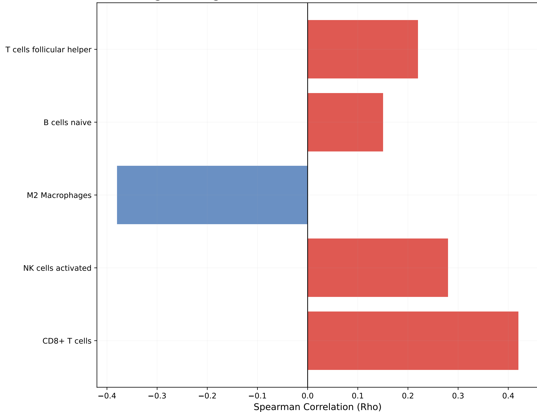
Figure 8: Signature Correlation with CIBERSORT Fractions
